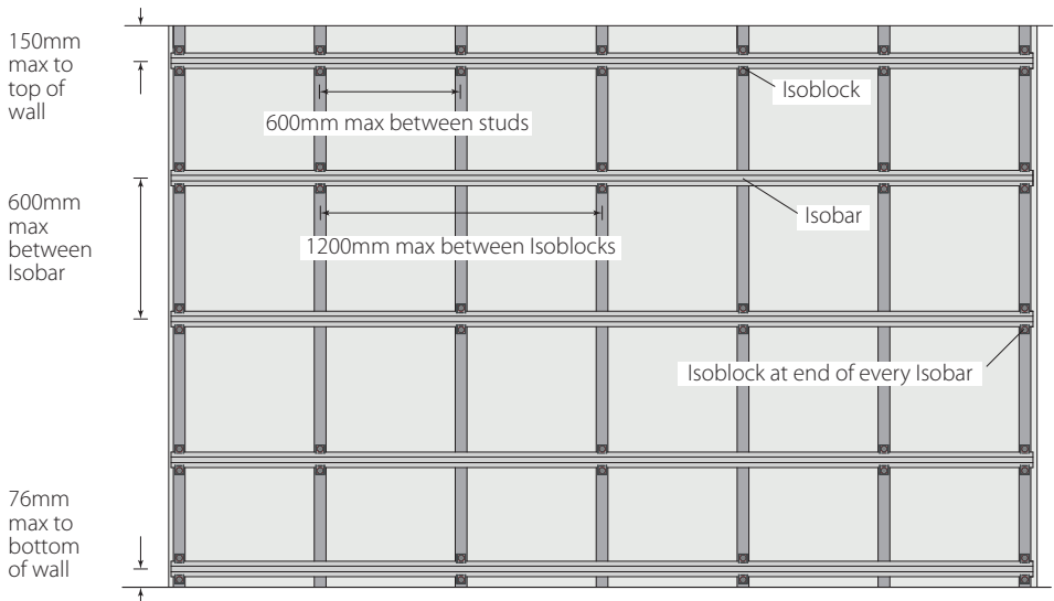
INSTALLATION - Walls
