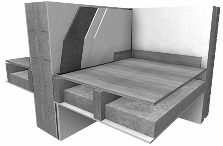
Re-Mat M20 on typical blockwork party wall with timber joist floor
